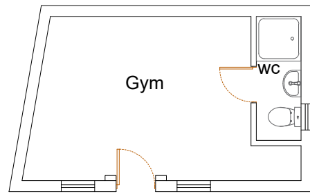
Proposed Outbuilding Floor Plan
