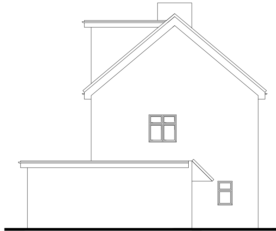
05 SIDE ELEVATION
